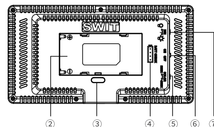
Fig.3 CL-15 Back view
