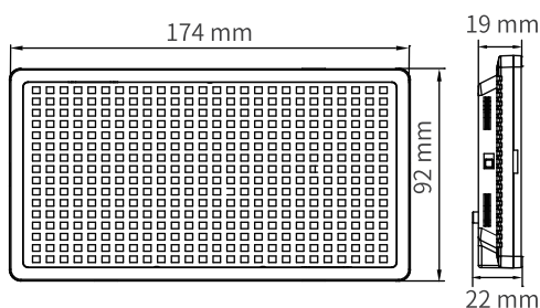
Fig.1 CL-15 Overall Dimension
